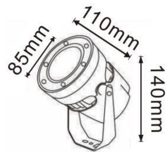
XYFLP-85-ZJ XYFLP-85H-ZJ
