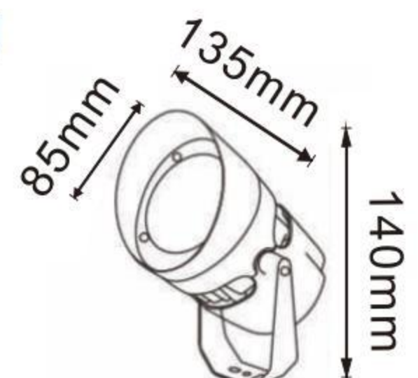
XYFLP-85-ZJ XYFLP-85H-ZJ
